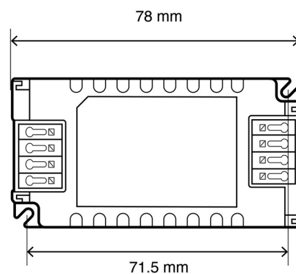
Dimension without strain relief
