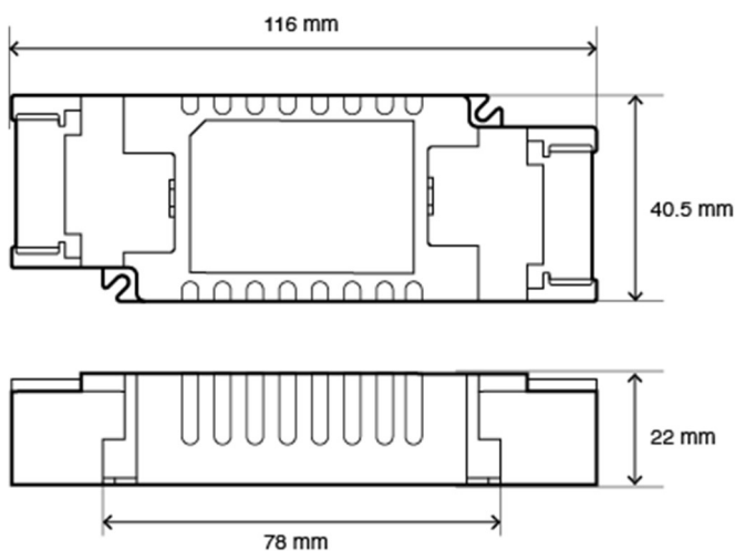
Dimension With strain relief
